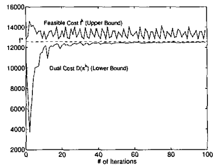
Fig. 1. Dual and Feasible Cost in the first example
