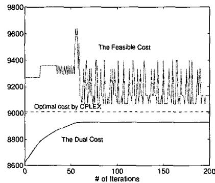
Fig. 2. Dual and Feasible Cost in the second example
